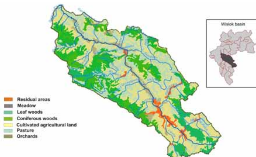
Fig. 2. Land use in the Stobnica basin; source: WAŁĘGA et al. [2009]
