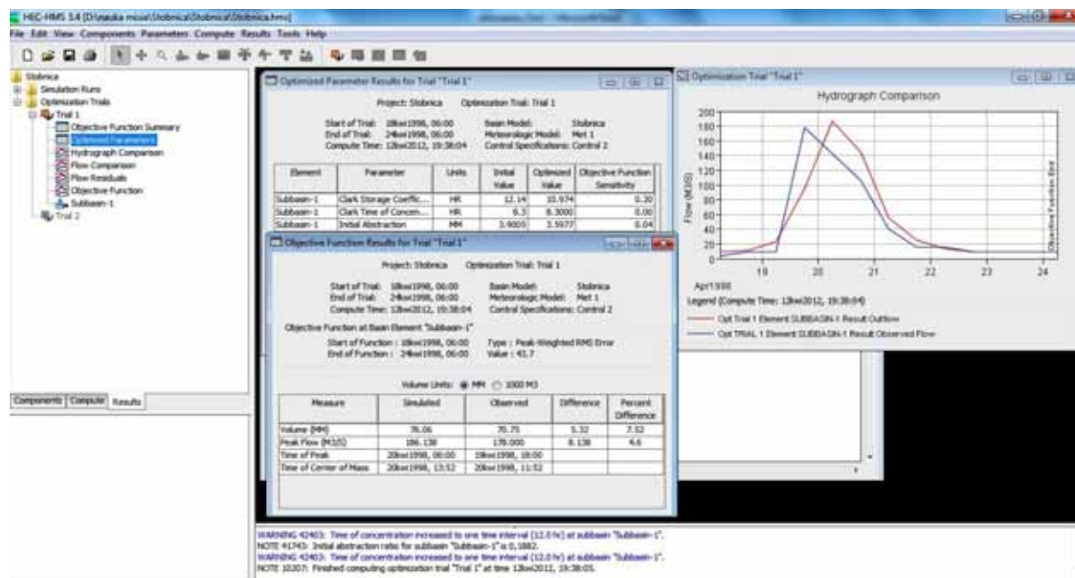
Fig. 3. Dialog screen with results of the IUH_Clark model parameter calibration; source: own study
