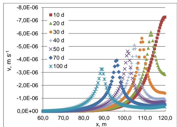
Fig. 6. Velocity distribution along the bottom of the channel on the upstream site (soil D); source: own study
