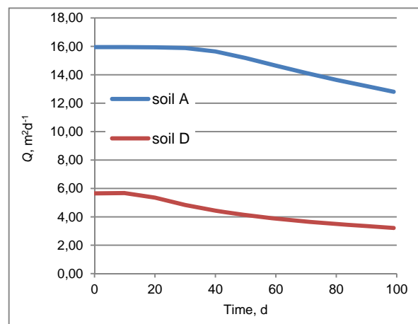
Fig. 3. Seepage flow; source: own study
