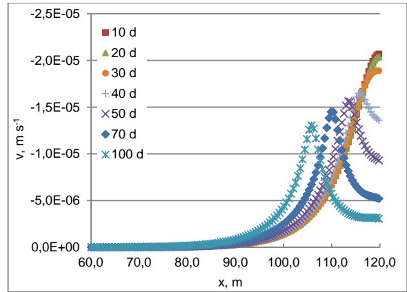
Fig. 5. Velocity distribution along the bottom of the channel on the upstream site (soil A); source: own study
