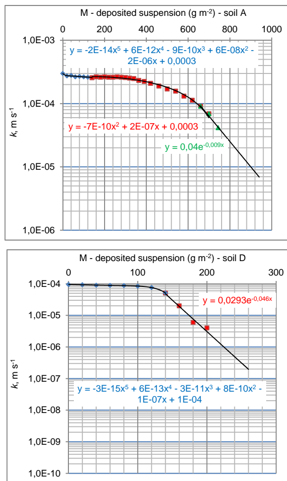
Fig. 2. Relation found between seepage coefficient k_1 and clogging clomatant mass M for soil A and D; source: own study based upon data obtained by SKOLASIŃSKA [2006]
