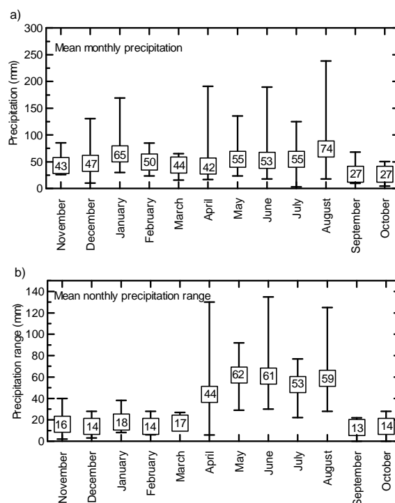
Fig. 7. Mean monthly precipitation sums (a) and mean monthly precipitation range (b); whiskers show extreme pixel values in particular months in years 2004–2008 registered in the Łasica catchment
