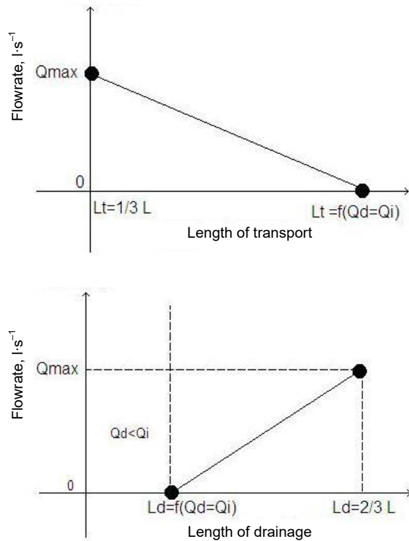
Fig. 8. Evolution of the throughput of a foggara depending on the length of transport and drainage; source: own elaboration
