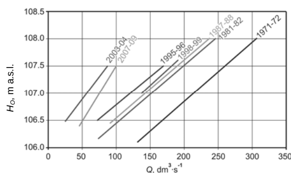
Fig. 4. Relationship between flow rate Q in the drainage canal in the Warzyna section and water elevation H_0 in the Odra in upper water section in the Brzeg Dolny barrage between 1971–2009; source: own elaboration
