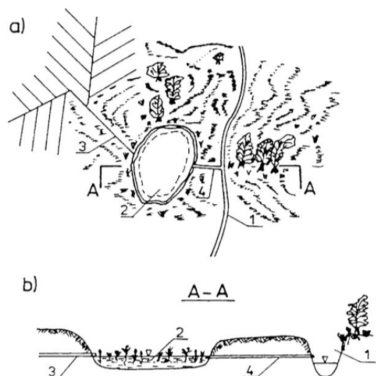
Fig. 8. A scheme of the biofilter located in the vicinity of a drainage water recipient: a) situation plan, b) A-A section; 1 – water course (drainage water recipient), 2 – dug pond covered by vegetation, 3 – outlet of the drainage water, 4 – discharge of purified water to the water course (open ditch or pipeline)
