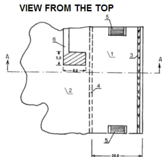
Fig. 3. Plan of the natural swimming pool; 1 – deep part (recreational), 2 – shallow part covered by aquatic plants, 3 – vertical wall, 4 – wall separating the shallow part from the deep one, 5 – stairs going down to the water, 6 – viewing platform
