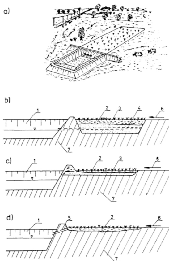
Fig. 7. A scheme of reservoir for preliminary surface runoff water purification: a) general view of the reservoir, b), c), d) cross sections of different types of reservoirs of verified construction; 1 – pond, 2 – initial pond (biofilter) of 20–30 cm depth covered by plants, 3 – filtration material (sand), 4 – drainage, 5 – pipeline draining water (or space in the crown of the dike), 6 – water flow direction, 7 – poorly permeable substratum
