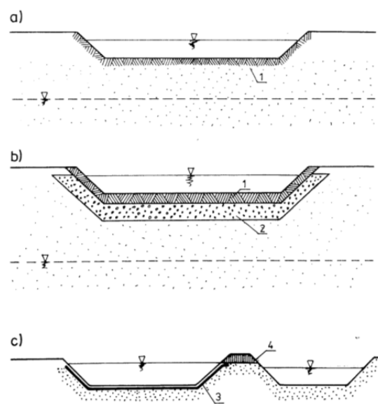
Fig. 9. Schemes of infiltration reservoirs: a) natural basin, b) filtration layer, c) infiltration reservoir with preliminary settling; 1 – soil, 2 – filtration layer, 3 – plastic sealing, 4 – overflow (pipeline)
