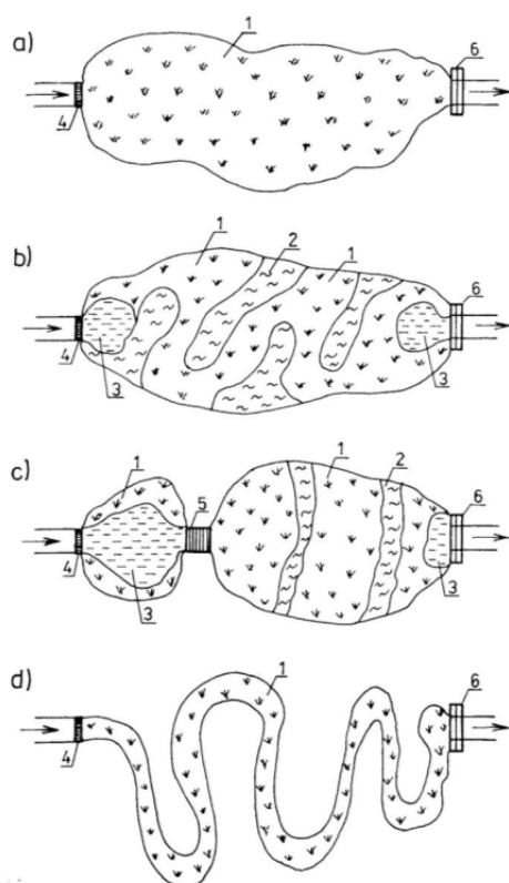
Fig. 6. Schemes of reservoirs (biofilters) for the purification of polluted water; a) one-chamber reservoir, b) reservoir with diverse surface, c) two-chamber reservoir, d) channel (ditch); 1 – surface of the reservoir covered by aquatic plants or grass, 2 – elevated areas of the reservoir or areas covered by higher vegetation, 3 – reservoir filled with water, 4 – inlet construction, 5 – rapid flow channel (cascade), 6 – outlet construction; source: CAMPBELL, OGEN [1999]
