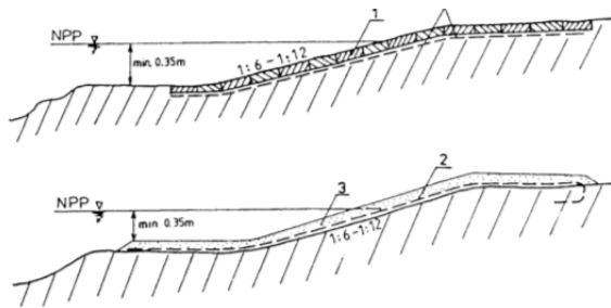
Fig. 1. Examples of a simple watering site construction: 1 – concrete slabs, rods or wooden boards, 2 – geotextiles, 3 – sand
