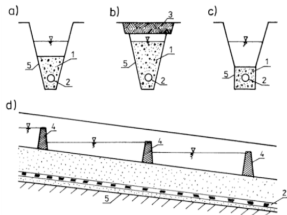
Fig. 11. Infiltration ditches scheme: a), b), c) cross sections, d) longitudinal section of the ditch a) and c); 1 – filtration material (gravel, stones), 2 – pipe drainage with filtration cover, 3 – turf, 4 – overflows, natural bottom (poorly permeable or impermeable) or sealed with plastic
