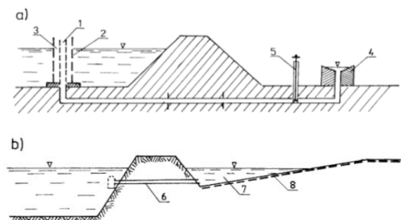
Fig. 2. Water intake from the pond for cattle watering scheme: a) reservoir, b) dug pond; 1 – perforated pipe of 10–15 cm diameter, 2 – perforated pipe of 50–200 cm diameter, 3 – coarse sand or gravel, 4 – drinking site of length depending on the number of cattle, 5 – valve, 6 – metal pipeline with metal stainer, 7 – waterhole, 8 – bottom strengthening such as geotextile
