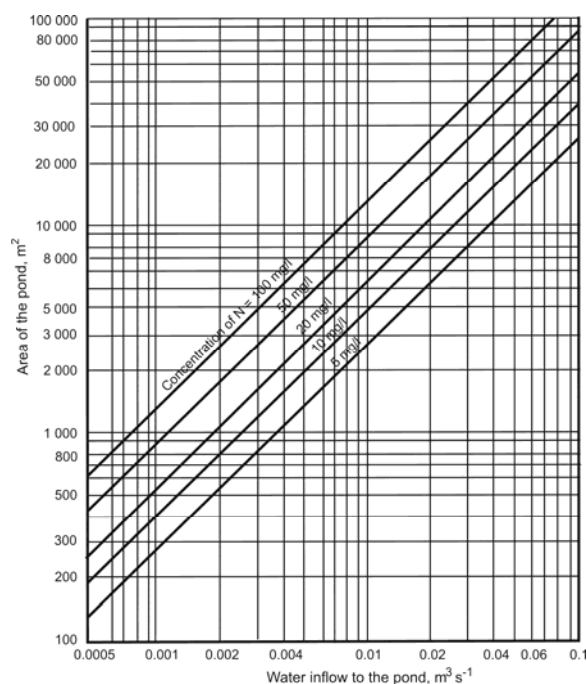
Fig. 5. A nomogram for determining the minimum size of the pond for water purification from nitrogen (average depth of 0.5 m)
