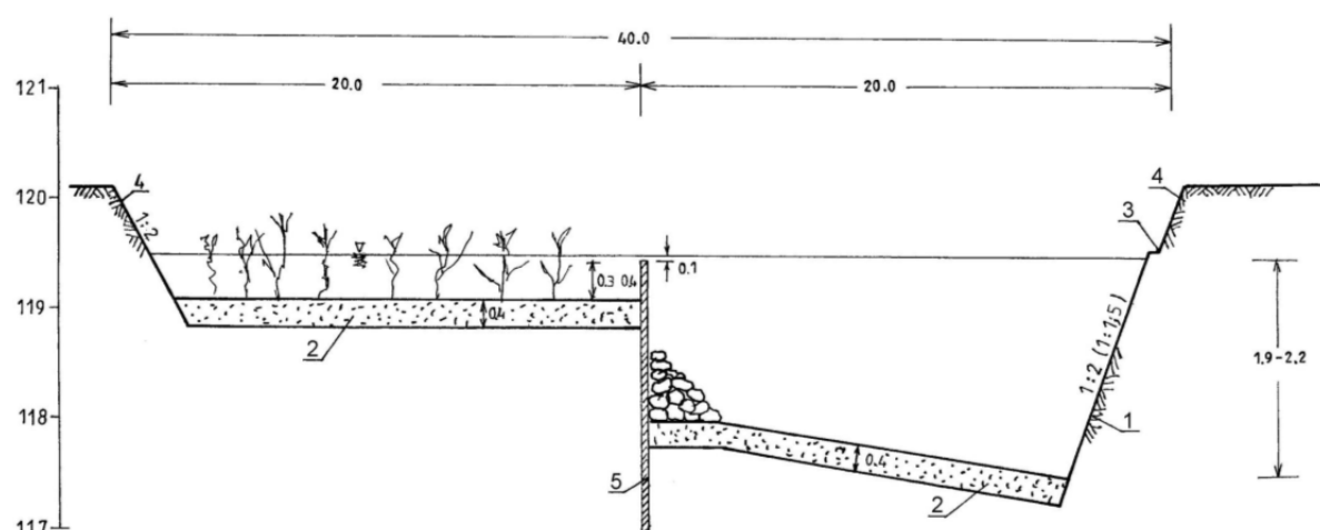
Fig. 4. A schematic cross section through the natural swimming pool; 1 – slope of the deep part of the pool, 2 – bottom (gravel, coarse sand), 3 – bench allowing a walk over the water table, 4 – slope covered by grass, 5 – wall separating the deep part of the pool from the shallow one
