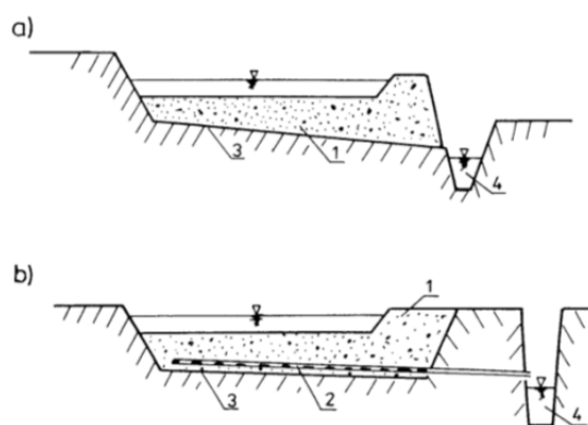
Fig. 10. Schemes of filtration basins: a) simple basin, b) drained basin; 1 – filtration material, 2 – drainage with a filter cover, 3 – natural bottom (impermeable or poorly permeable) or sealed with plastic, 4 – infiltrating water recipient (water course, pond, channel, pipeline, etc.)
