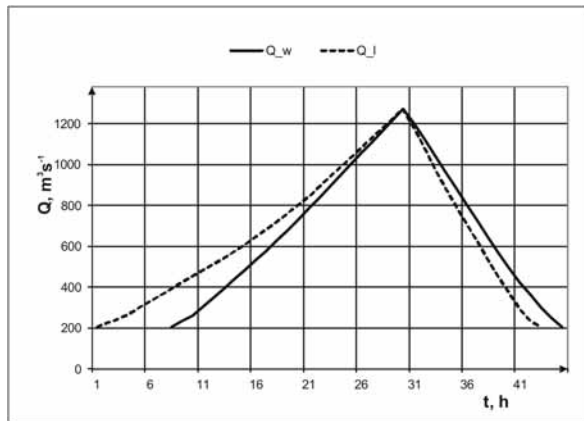
Fig. 12. Hypothetical hydrograph at the Koszyce Wielkie water-gauge cross-section on the Biała River for Q_{p=1\%} developed by the Cracow method based on the limnigraph data ( Q_l hydrograph) and the staff-gauge data ( Q_w hydrograph); source: own study
