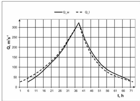
Fig. 11. Hypothetical hydrograph at the Nowy Sącz water-gauge cross-section on the Kamiénica River for Q_{p=1\%} developed by the Cracow method based on the limnigraph data ( Q_l hydrograph) and the staff-gauge data ( Q_w hydrograph); source: own study
