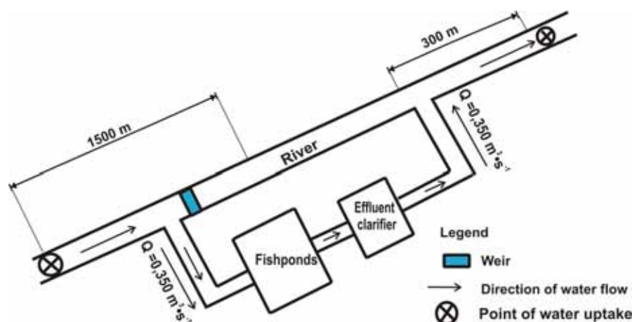
Fig. 2. Detailed scheme of fish farm; source: own study
