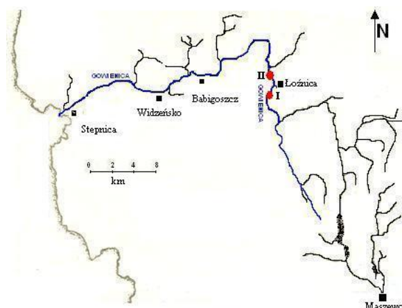
Fig. 1. Catchment basin of the Gowienica River with marked sites of water sampling upstream (I) and downstream (II) the rainbow trout farm in Łoźnica; source: own study
