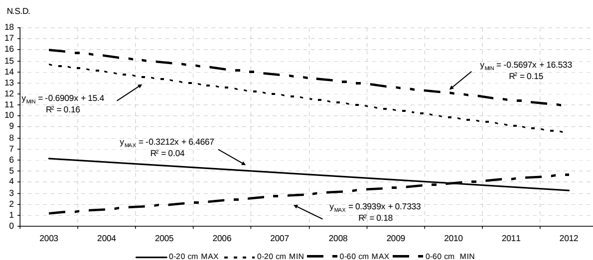
Fig. 4. Tendencies of the occurrence of decades (N.S.D.) of maximum and minimum values of soil water reserves in soil layers 0–20 and 0–60 cm in summer half-year of the period 2003–2012; source: own study
