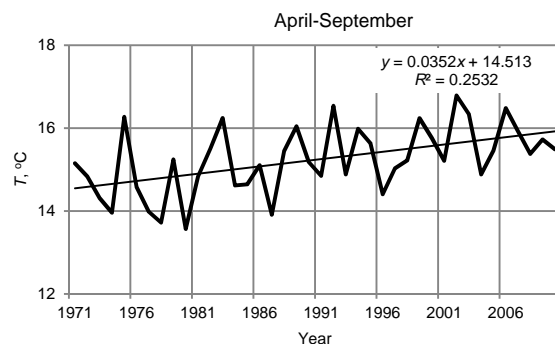
Fig. 1. Mean air temperature T (°C) in the growing season (April–September) in the meteorological station Bydgoszcz–ITP in 1971–2010; source: own study
