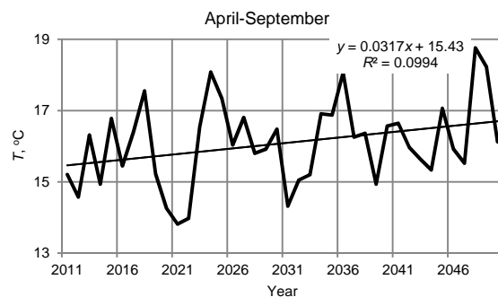
Fig. 2. Predicted mean air temperature T (°C) in the growing season in Bydgoszcz region in the years 2011–2050; source: own study
