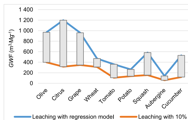
Fig. 3. Effect of N leaching with \alpha = 10\% and regression model at GWF ; source: own study
