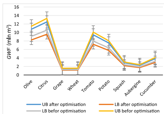
Fig. 4. Upper and lower bound of grey water footprint ( GWF ) before and after optimisation; LB = lower bound, UB = upper bound; source: own
