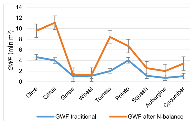
Fig. 2. The effect of N-fertilisers application rate of grey water footprint ( GWF ) before and after N-balance for studied crop; source: own study
