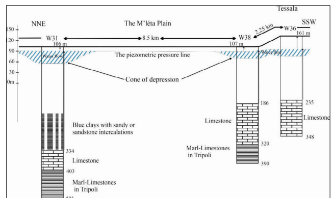
Fig. 4. Load of the water table in relation to the aquifer formations of the M'leta Plain; source: own elaboration
