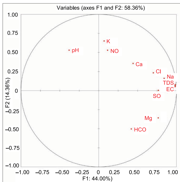
Fig. 6. Correlation circles for factors F1–F2; source: own study
