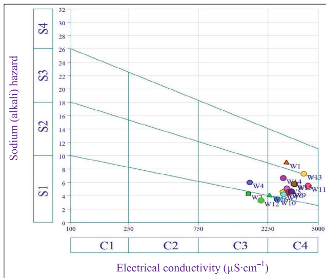
Fig. 10. Irrigation water quality based on sodium adsorption ratio; S1 = low sodium hazard, S2 = medium sodium hazard, S3 = high sodium hazard, S4 = very high sodium hazard, C1 = non-saline, C2 = slightly saline, C3 = moderately saline, C4 = very saline; source: own study
