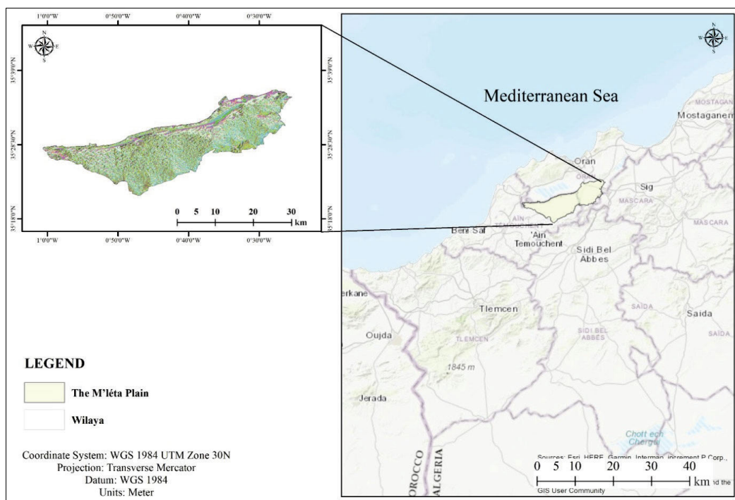
Fig. 1. Study area location; source: own elaboration
