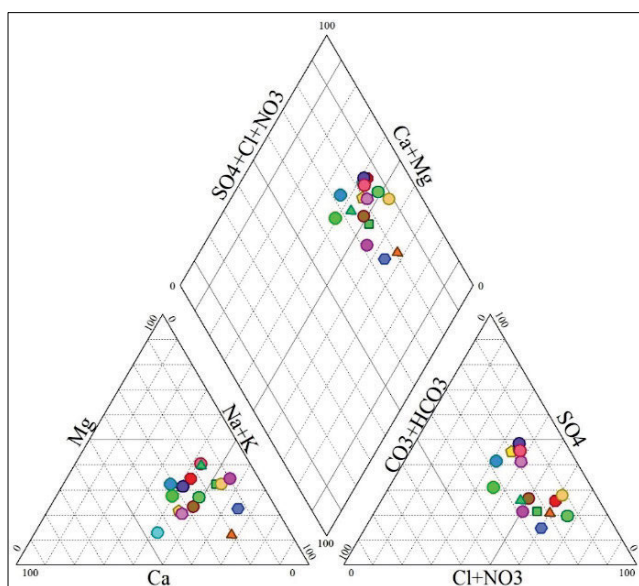
Fig. 8. Piper diagram of the Mio-Pliocene complex aquifer of the M'leta plain; source: own study
