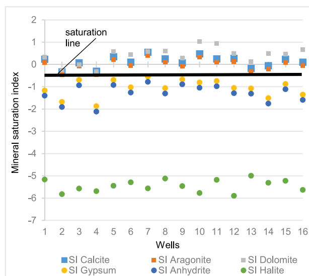
Fig. 9. Variation of the saturation index of the indicated minerals: carbonate minerals, gypsum, and halite; source: own study
