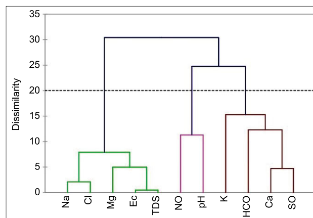
Fig. 7. Dendrogram of examined variables; source: own study
