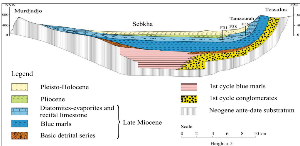
Fig. 3. Interpretative hydrogeological section of the basin of the great Sebka of Oran; source: Hassani (1987), modified
