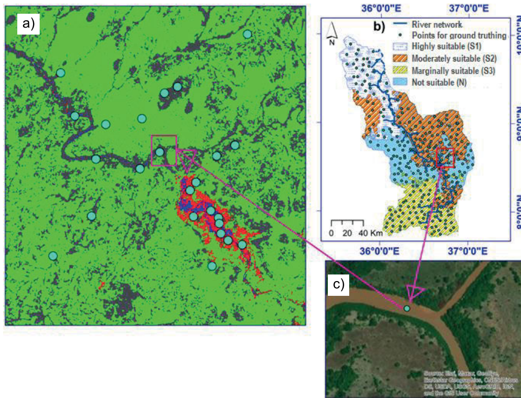
Fig. 9. Ground truth data based validated surface irrigation potential zones: a) supervised LULC classification, b) explored surface irrigation potential zones for MCA, c) base map for ground truthing for explored potential zones; source: own study
