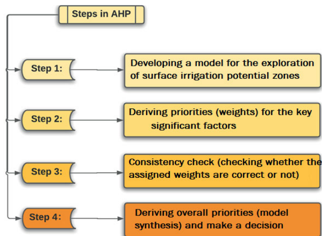
Fig. 2. The detailed steps in the analytic hierarchy process (AHP) during making a decision; source: own elaboration
