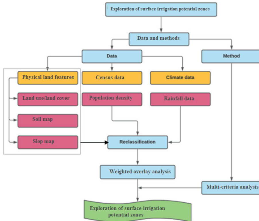
Fig. 7. Surface irrigation potential zones exploration; source: own study
