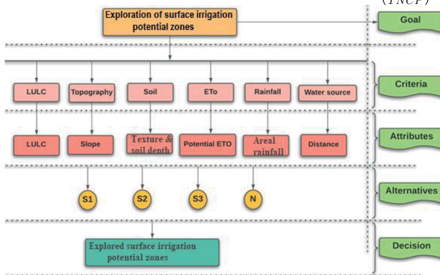
Fig. 6. Hierarchical framework of surface irrigation potential zones exploration; source: own study
