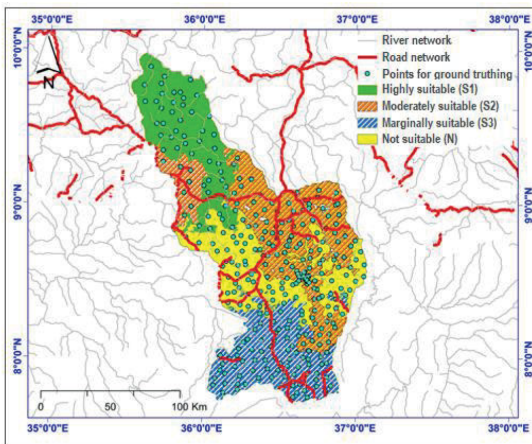
Fig. 8. Map of the explored surface irrigation potential zones; source: own study
