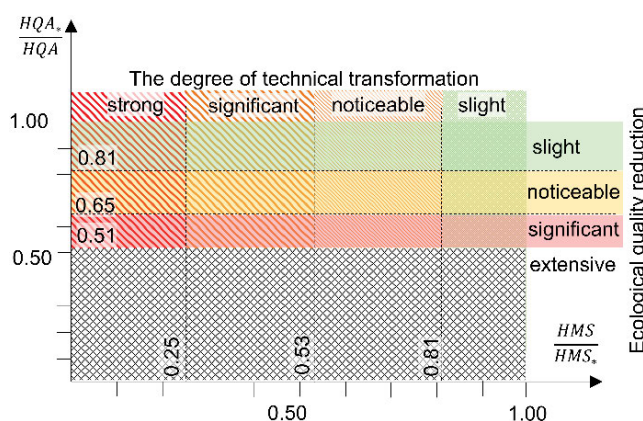
Fig. 4. Diagram for assessing the impact of the river section regulation on its hydromorphological status; HQA, HQA*, HMS, HMS* as in Fig. 3; source: own elaboration
