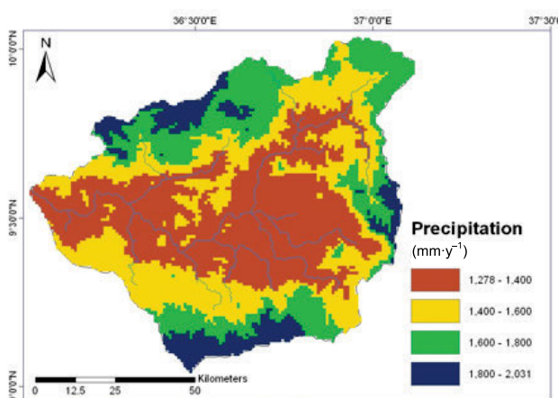
Fig. 3. Rainfall distribution in Anger sub-basin; source: Nekemte... [2015]
