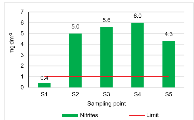
Fig. 8. Spatial evolution of nitrites (NO 2 - ); source: own study
