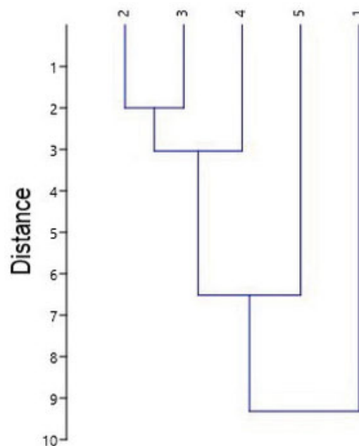
Fig. 3. Results of cluster analysis based on the principle of similarity between five aquifers: 1 = the Quaternary (anthropogenic) stage, 2 = the Apsheronian stage, 3 = the Akchaglyian stage, 4 = Kuyalnician stage, 5 = the Cimmerian stage; source: own study
