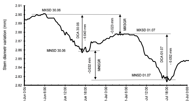
Fig. 1. Criteria for determining the start of watering; MXSD = maximum daily stem diameter, MNSD = minimum daily stem diameter, DCA = daily contraction amplitude, MXSGR = maximum daily stem growth rate, MNSGR = minimum daily stem growth rate; source: own study
